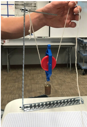
Movable Pulley:
